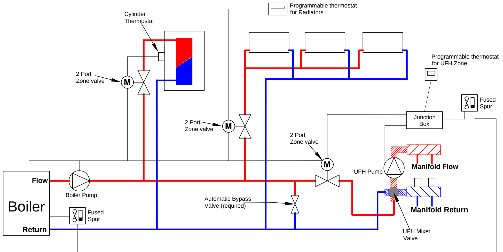
Typical Single Zone Underfloor on a S-Plan System
