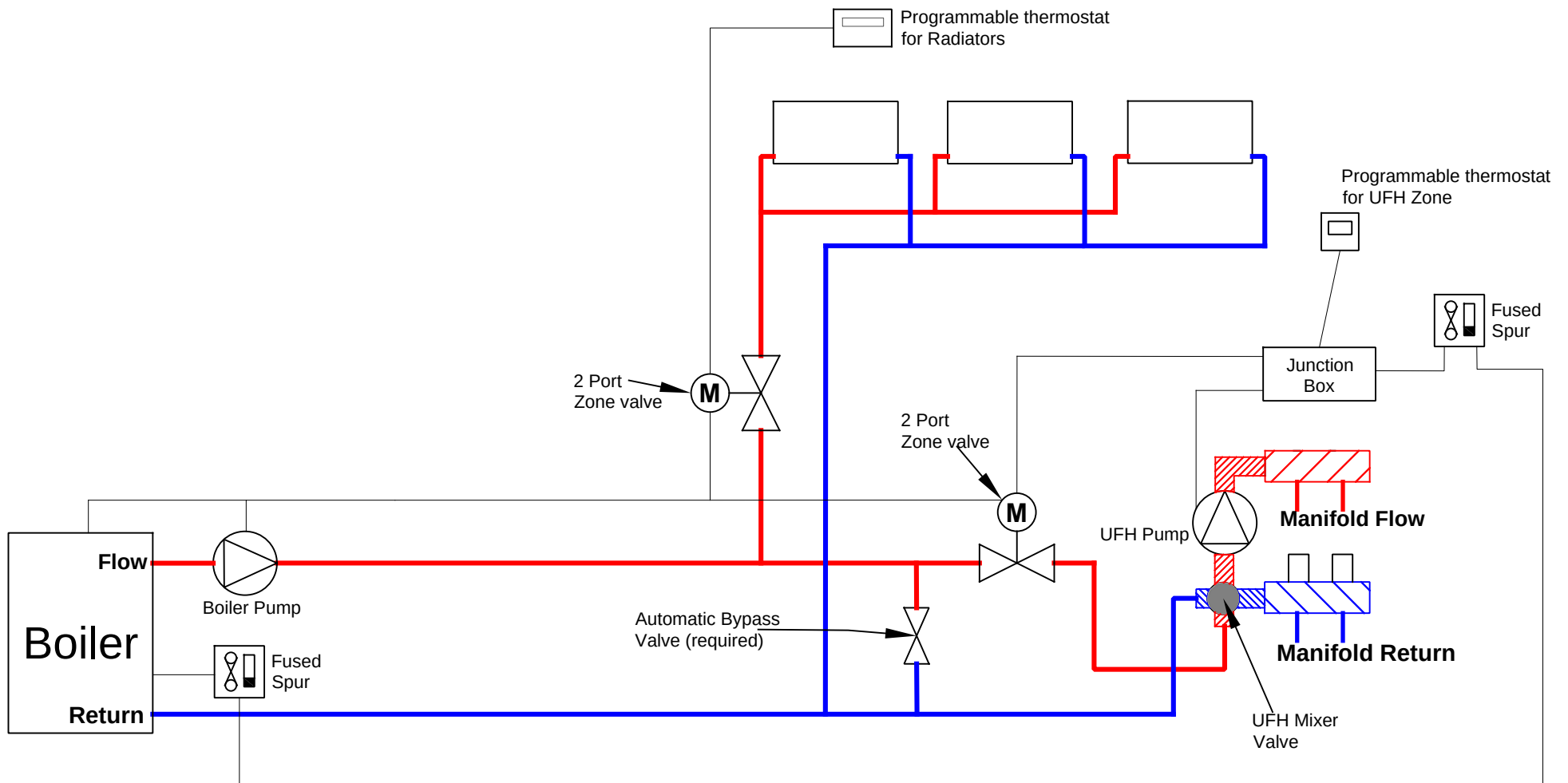
Typical Single Zone Underfloor on a S-Plan Combi System
