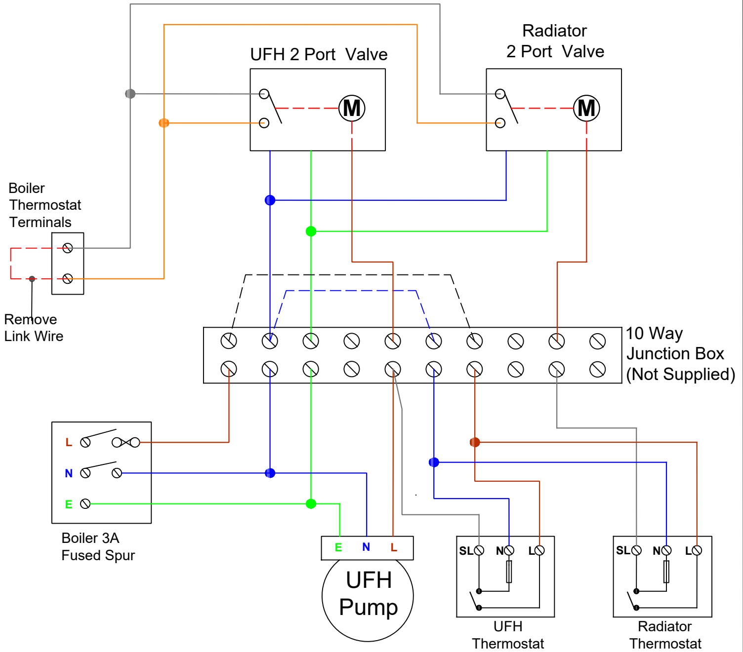
Wiring Using 2 Port Valves ( S Plan )
